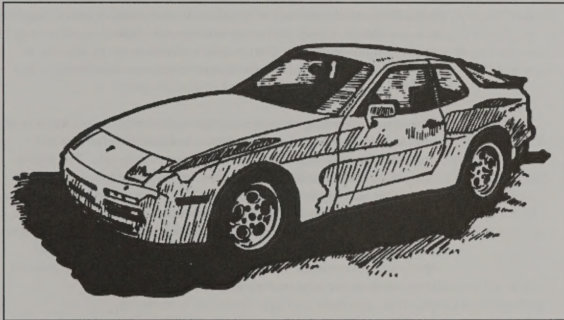
Figure 2. Interdisciplinary.
